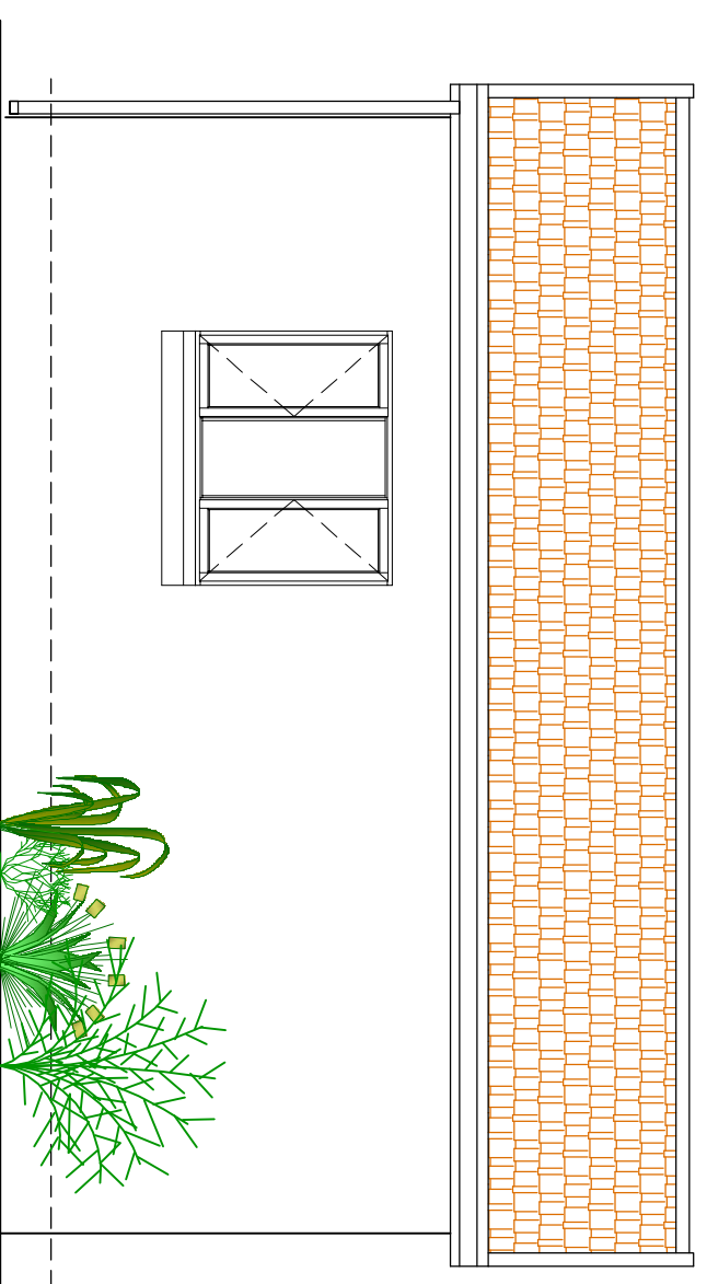
SIDE ELEVATION 1:50
